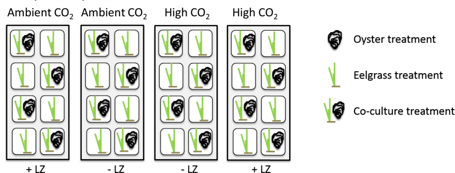
FIG. 2. Experimental design for phase I (A) and phase II (B) of our experiment. p\text{CO}_2 was manipulated at the level of the cooler (bigger rectangles), while biological treatments (smaller squares) were replicated within coolers. Thus, in phase I, there were a total of 45 experimental units (smaller squares) which represented nine experimental treatments replicated five times each. In phase II, there were a total of 32 experimental units (smaller squares), representing eight experimental treatments replicated four times each. For all analyses, measurements were averaged within the level of the experimental unit (small squares) and a random effect for the cooler was included in order to account for the non-independence of replicates within the coolers.
